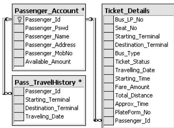
Figure 1 ERD of the Ticket Reservation
